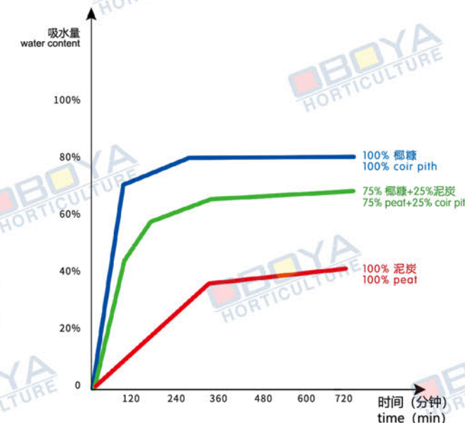
不同基质的吸水程度对比 Comparisons of the water absorbing capacities of different substrates
